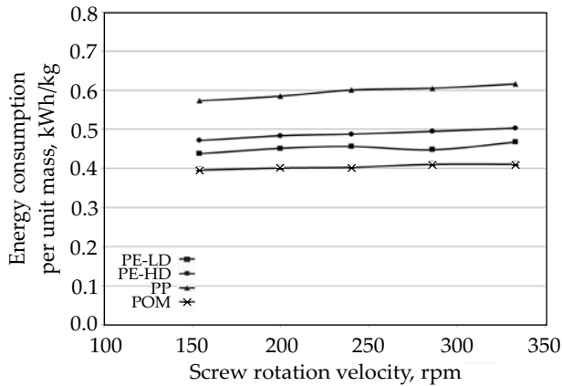
Fig. 9. SEC in injection molding process at variable screw rotation velocity
